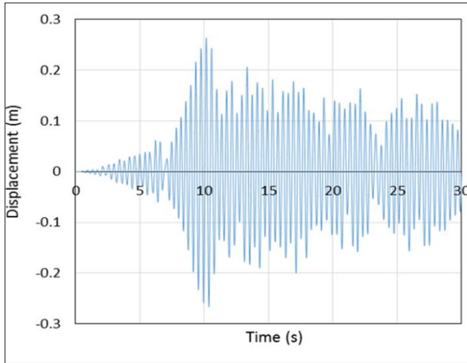
Figure 8. X-direction displacement of the top of the arrester for the hard mounted case.
