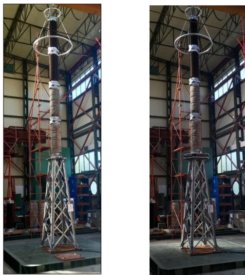
Figure 10. Test setups used of hard mounted case (left), elastically mounted case (right).
