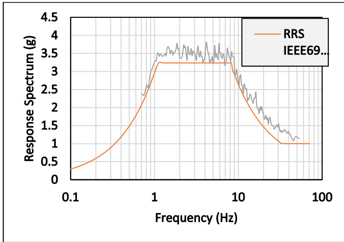
Figure 4. Shock response spectrum of 1 g time history input in X-direction
