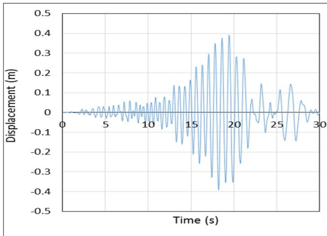
Figure 9. X-direction displacement of the top of the arrester for the elastically mounted case.
