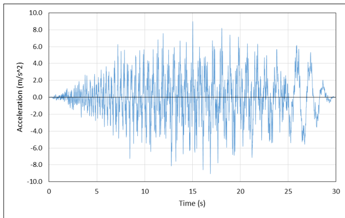
Figure 5. 1 g time history input in X-direction
